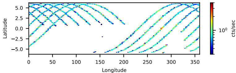
60161678002 FPMa: No SAA Filter 27.94-ks, 100%
