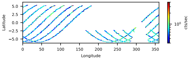
60161511002 FPMB: No SAA Filter 22.17-ks, 100%
