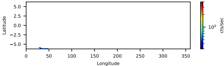
60161352001 FPMB: No SAA Filter 0.28-ks, 100%
