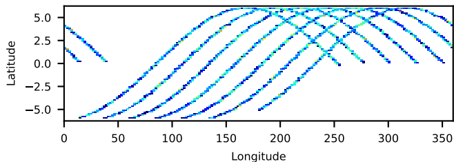
60161261002 FPMa: No SAA Filter 26.54-ks, 100%
