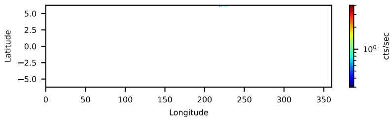
60160702001 FPMA: No SAA Filter 0.13-ks, 100%
