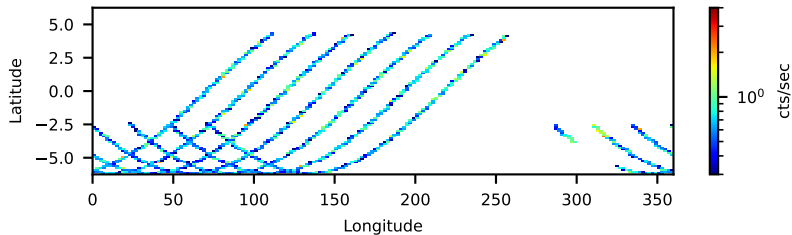
60160178002 FPMA: No SAA Filter 20.40-ks, 100%
