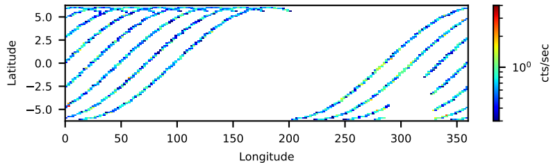
60061220002 FPMB: No SAA Filter 21.97-ks, 100%
