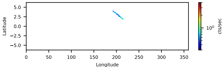
60061041001 FPMB: No SAA Filter 0.34-ks, 100%
