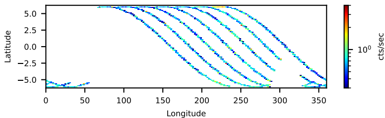
31002002008 FPMB: No SAA Filter 19.70-ks, 100%
