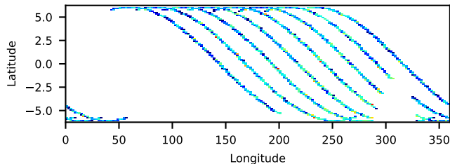
31002002006 FPMB: No SAA Filter 22.77-ks, 100%
