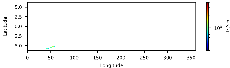
30902041005 FPMB: No SAA Filter 0.29-ks, 100%
