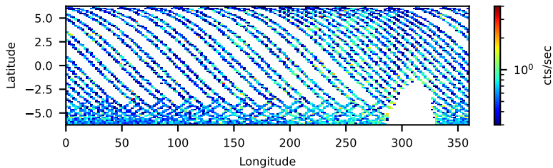
30901014002 FPMB: No SAA Filter 104.98-ks, 100%
