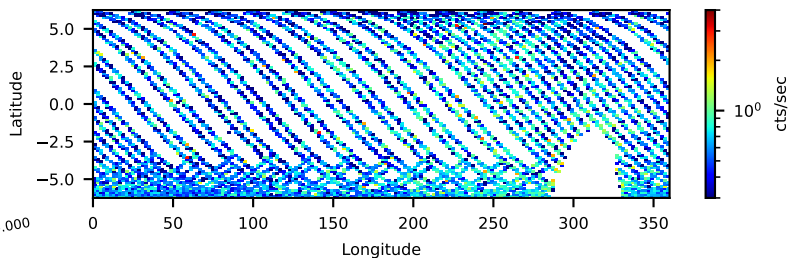
30901014002 FPMB: No SAA Filter 104.98-ks, 100%
