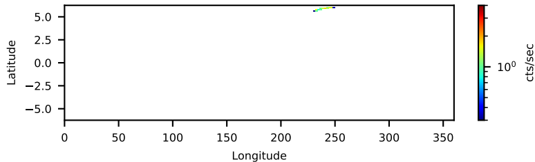
30901002001 FPMA: No SAA Filter 0.27-ks, 100%
