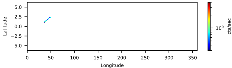
30801018001 FPMA: No SAA Filter 0.21-ks, 100%
