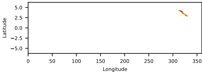
30702013008 FPMB: No SAA Filter 0.26-ks, 100%
