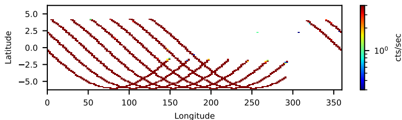
11002306004 FPMB: No SAA Filter 22.88-ks, 100%
