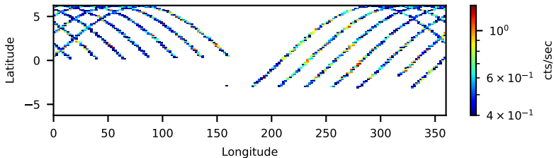
91002609002: 3 to 120 keV
