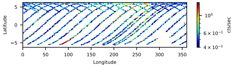
91002520004: 3 to 120 keV
