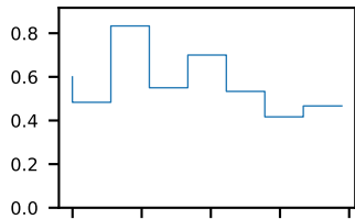
60-s bins
