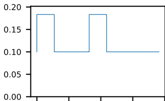
60-s bins
