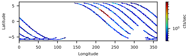
91002305002: 3 to 120 keV
