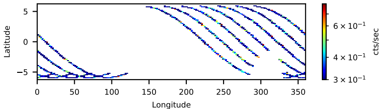
91002305002: 30 to 120 keV
