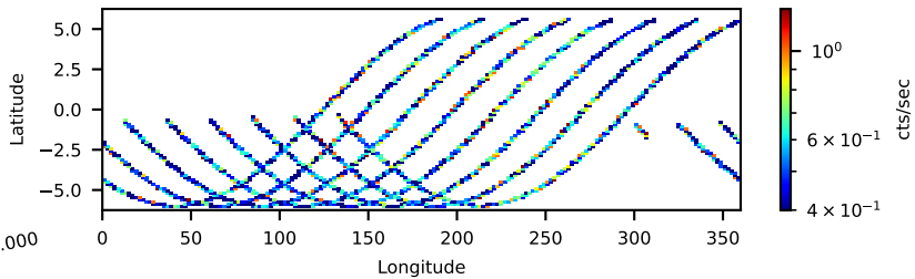
91001601002: 3 to 10 keV
