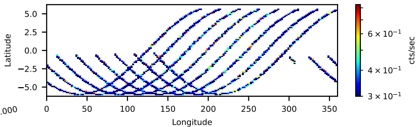
91001601002: 30 to 120 keV
