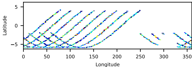
91001314002: 3 to 10 keV
