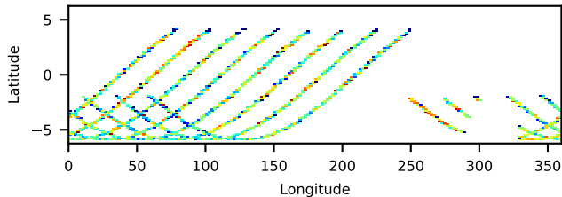
91001314002: 3 to 120 keV
