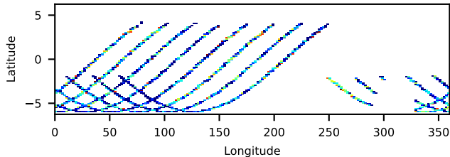
91001314002: 30 to 120 keV
