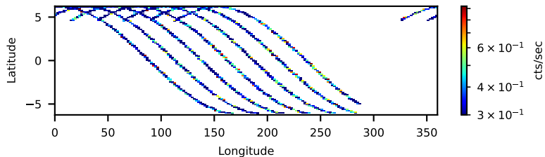
90902329002: 30 to 120 keV
