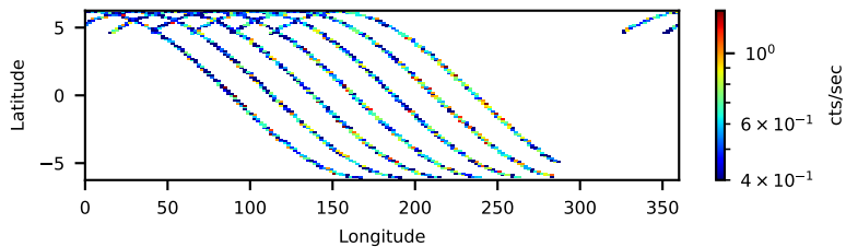
90902329002: 3 to 120 keV
