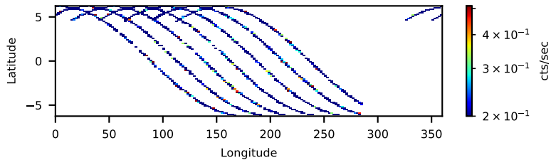
90902329002: 3 to 10 keV
