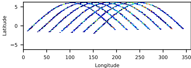
90902326002: 30 to 120 keV
