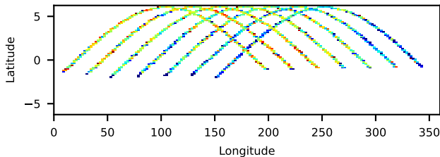
90902326002: 3 to 120 keV
