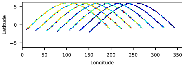
90902326002: 3 to 10 keV
