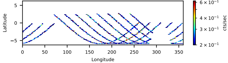
90901615002: 3 to 10 keV
