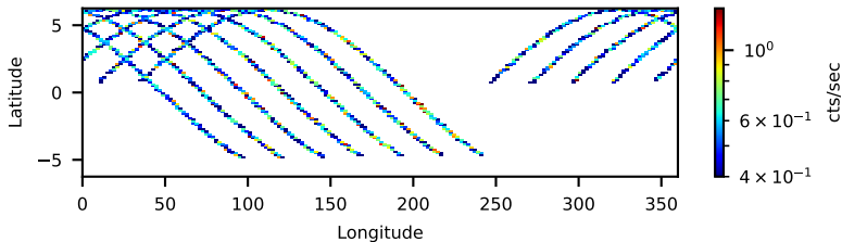
90901614002: 3 to 120 keV
