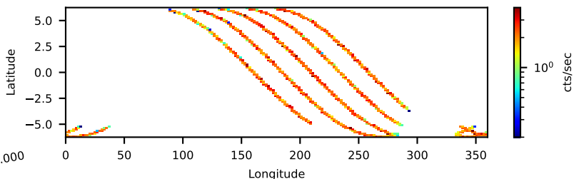
90901528002: 30 to 120 keV
