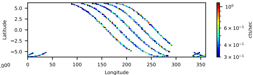
90901528002: 30 to 120 keV
