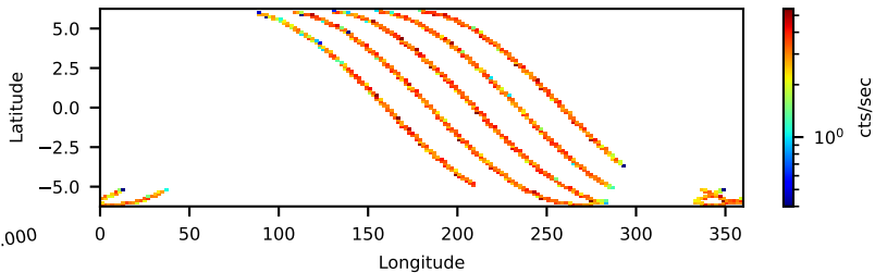
90901528002: 3 to 10 keV
