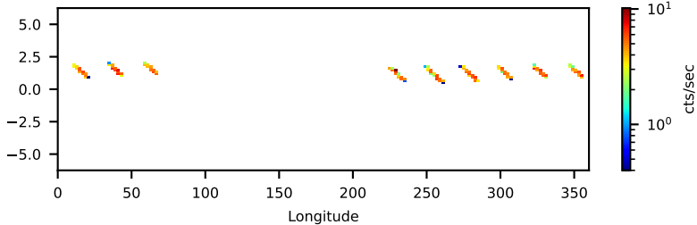
90901335002: 3 to 10 keV
