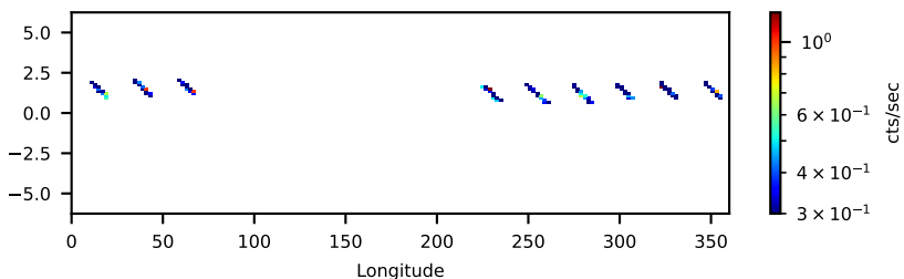
90901335002: 30 to 120 keV
