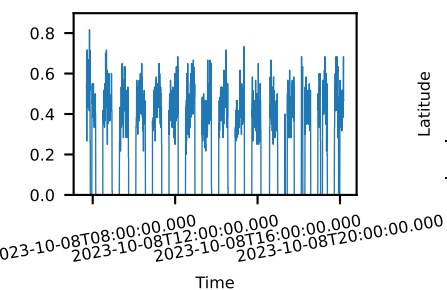
60-s bins
