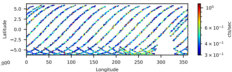
90901331002: 30 to 120 keV
