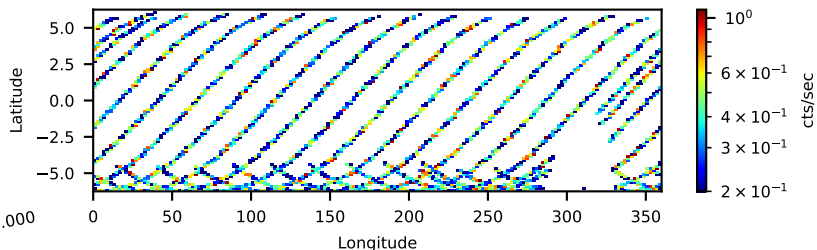
90901331002: 30 to 120 keV
