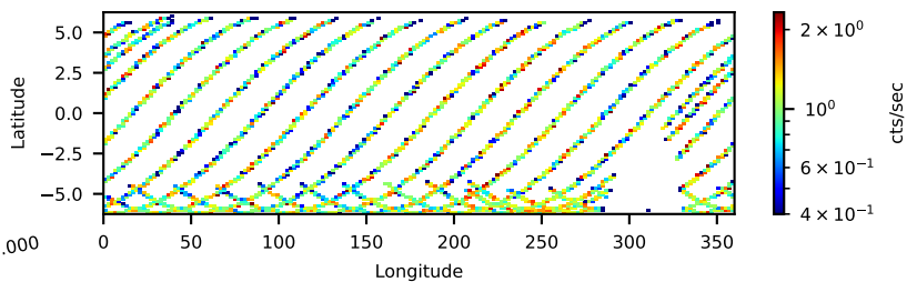
90901331002: 3 to 10 keV
