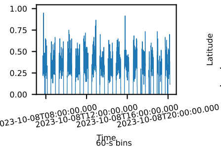
60-s bins
