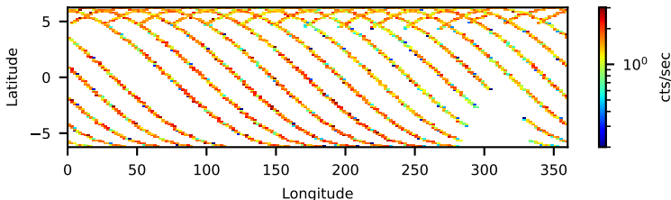
90901327002: 3 to 10 keV
