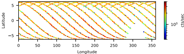
90901327002: 3 to 120 keV
