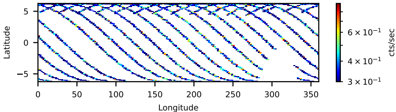
90901327002: 30 to 120 keV
