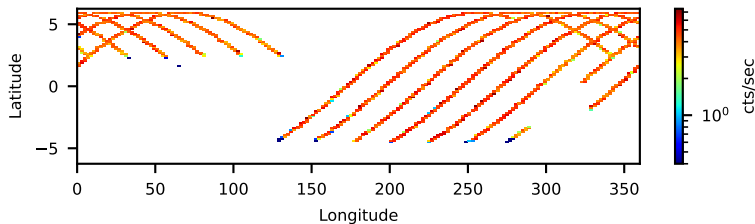
90802327002: 3 to 120 keV
