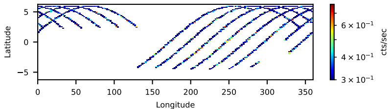
90802327002: 30 to 120 keV
