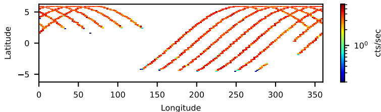
90802327002: 3 to 10 keV
