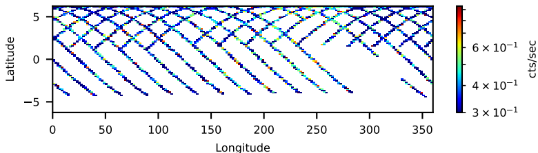
90802306002: 30 to 120 keV
