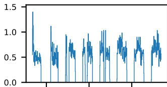
60-s bins
