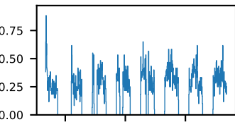
60-s bins
