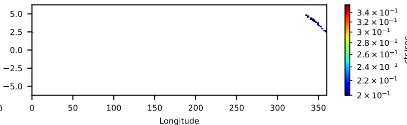
90701344001: 30 to 120 keV
