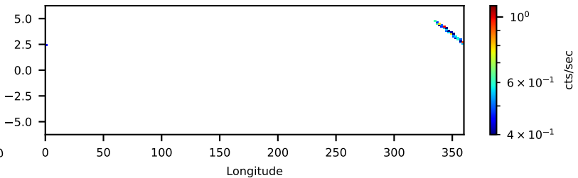
90701344001: 3 to 10 keV
