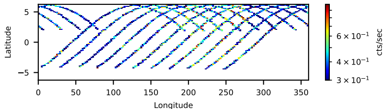
90701341002: 30 to 120 keV
