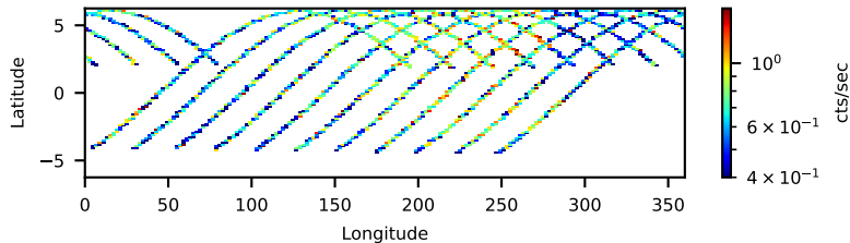
90701341002: 3 to 120 keV
