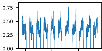
60-s bins
