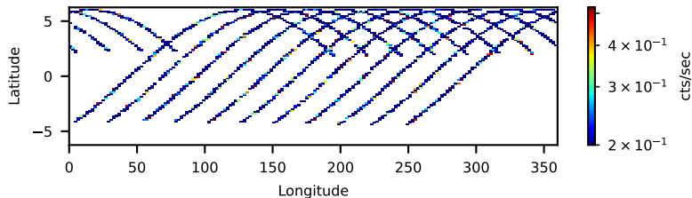
90701341002: 3 to 10 keV
