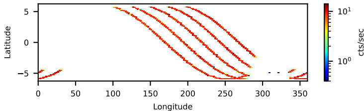
90601335002: 3 to 120 keV
