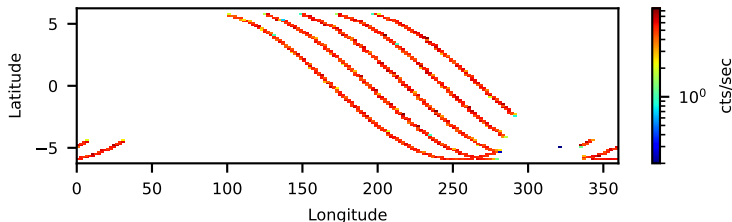
90601335002: 3 to 10 keV
