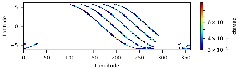
90601335002: 30 to 120 keV
