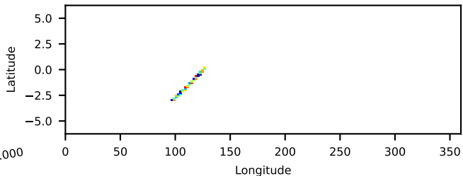
90502352001: 30 to 120 keV
