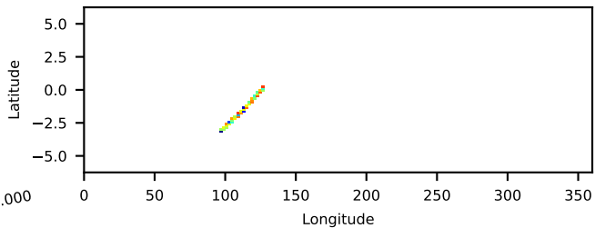
90502352001: 3 to 10 keV
