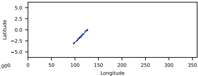
90502352001: 30 to 120 keV
