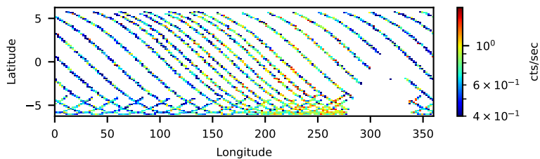
90501351002: 3 to 120 keV
