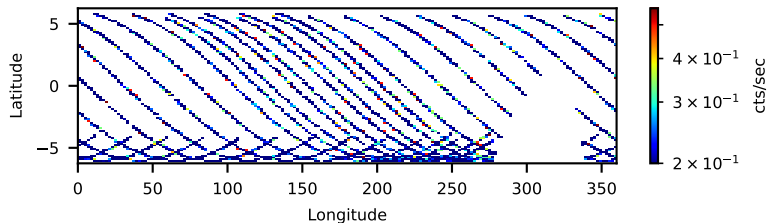
90501351002: 3 to 10 keV
