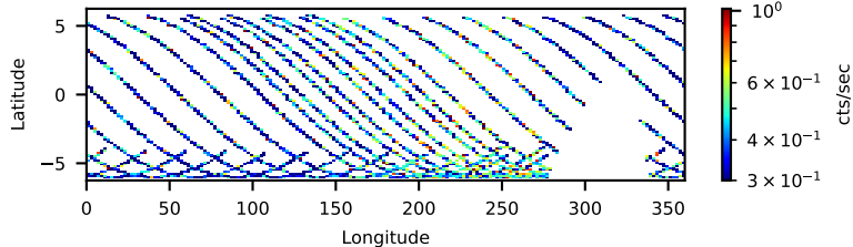
90501351002: 30 to 120 keV
