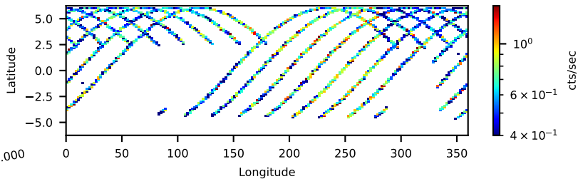
90402637002: 3 to 10 keV
