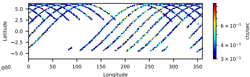
90402637002: 30 to 120 keV
