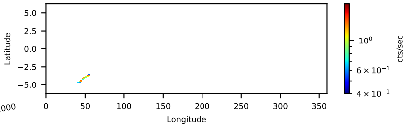
90401371001: 3 to 10 keV
