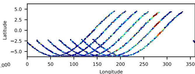
90301618004: 30 to 120 keV
