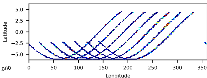
90301618004: 30 to 120 keV
