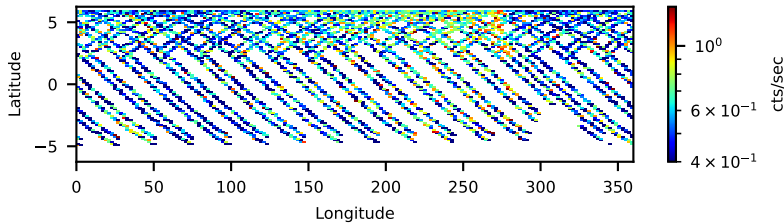
81001646002: 3 to 120 keV
