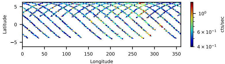
80902632004: 3 to 120 keV
