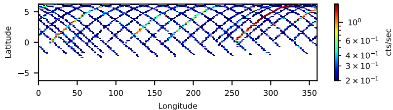
80902503002: 3 to 10 keV
