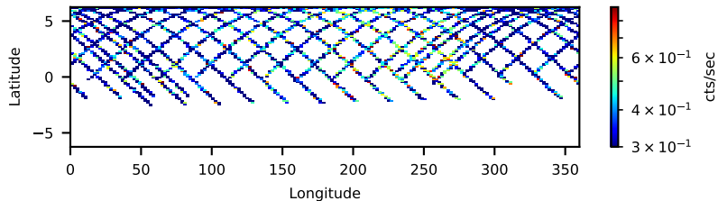
80902503002: 30 to 120 keV
