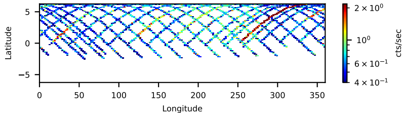
80902503002: 3 to 120 keV
