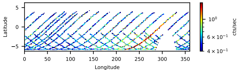
80901309002: 3 to 120 keV
