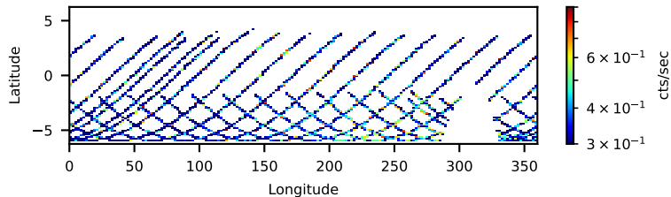
80901309002: 30 to 120 keV
