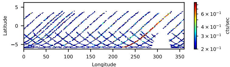
80901309002: 3 to 10 keV
