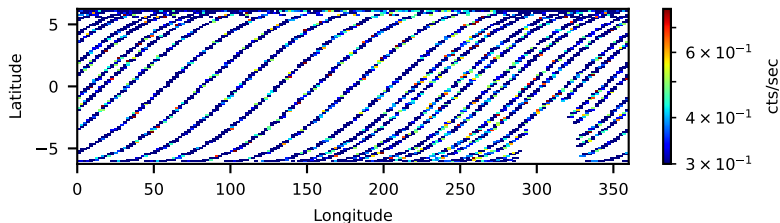
80802652004: 30 to 120 keV
