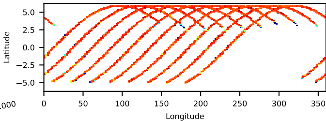
80802346002: 3 to 10 keV
