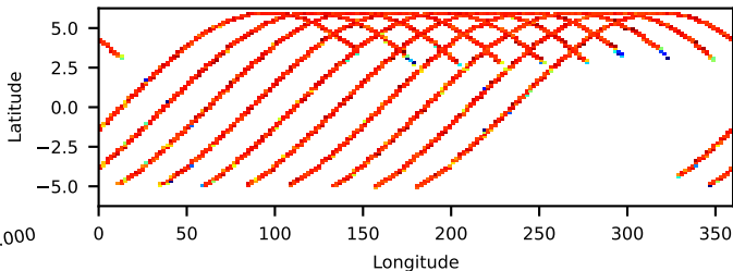
80802346002: 30 to 120 keV
