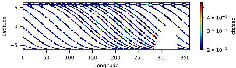
80801603002: 3 to 10 keV
