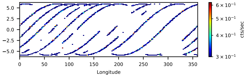
80801327002: 30 to 120 keV
