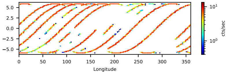
80801327002: 3 to 10 keV
