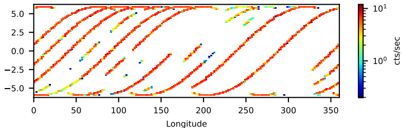
80801327002: 30 to 120 keV
