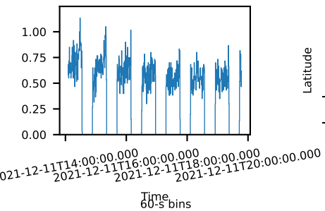
60-s bins
