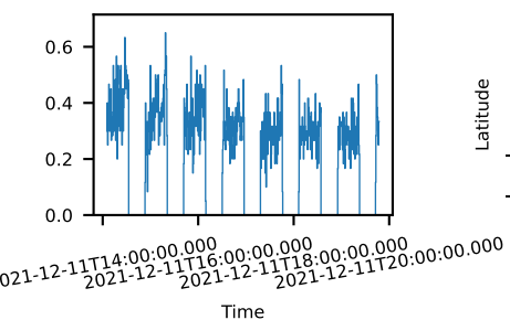
60-s bins
